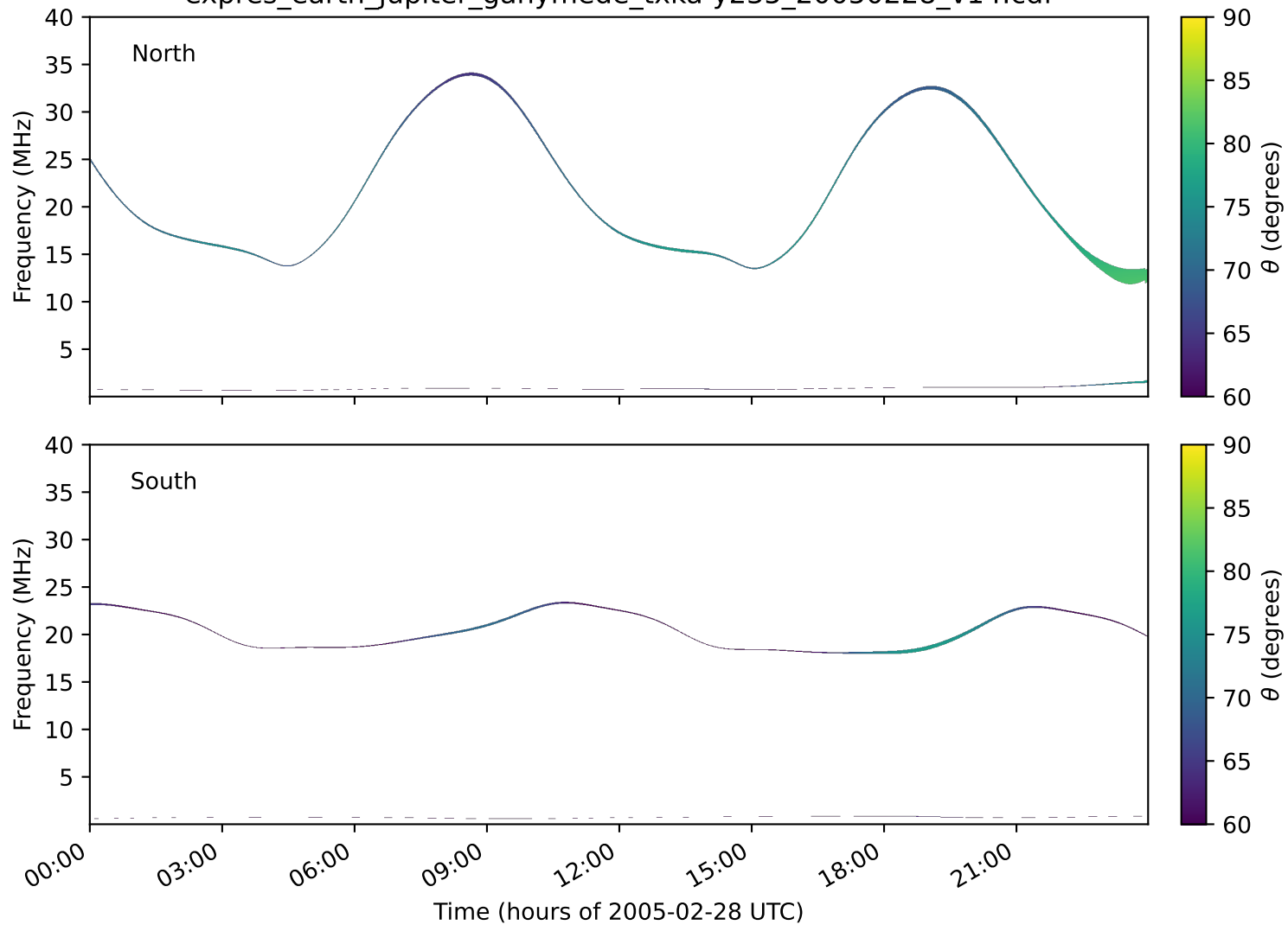
expres_earth_jupiter_ganymede_txka-y235_20050228_v14.cdf
