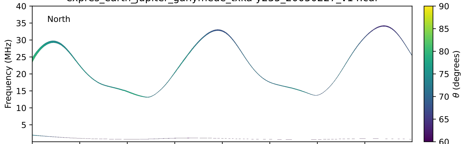
expres_earth_jupiter_ganymede_txka-y235_20050227_v14.cdf
