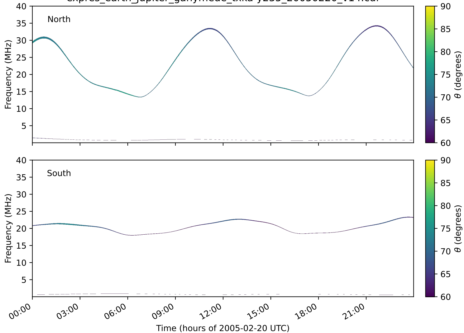
expres_earth_jupiter_ganymede_txka-y235_20050220_v14.cdf
