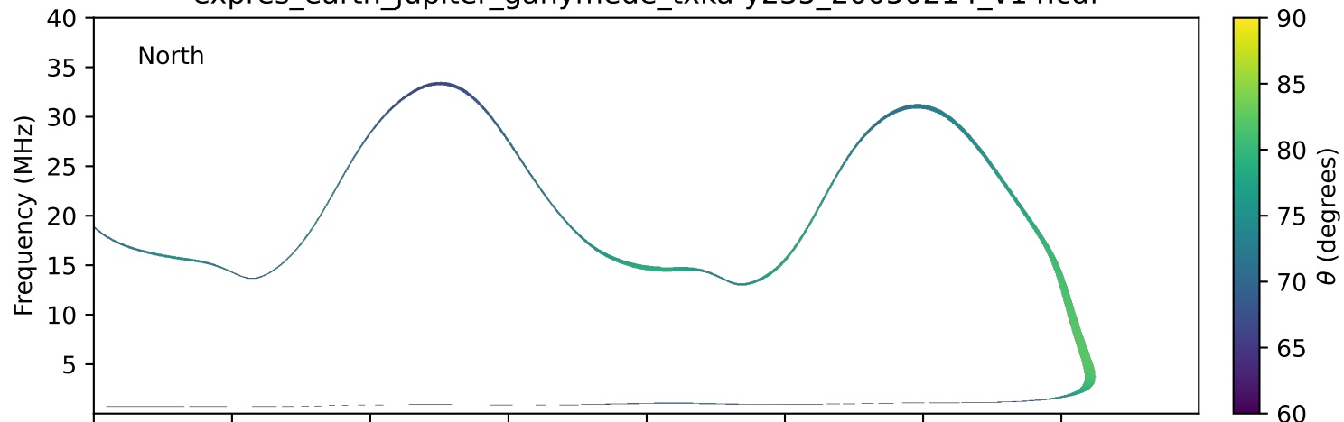
expres_earth_jupiter_ganymede_txka-y235_20050214_v14.cdf
