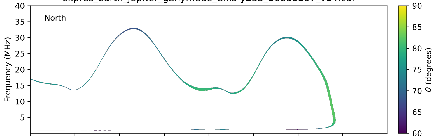
expres_earth_jupiter_ganymede_txka-y235_20050207_v14.cdf
