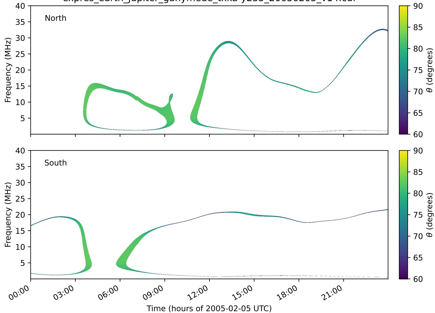
expres_earth_jupiter_ganymede_txka-y235_20050205_v14.cdf
