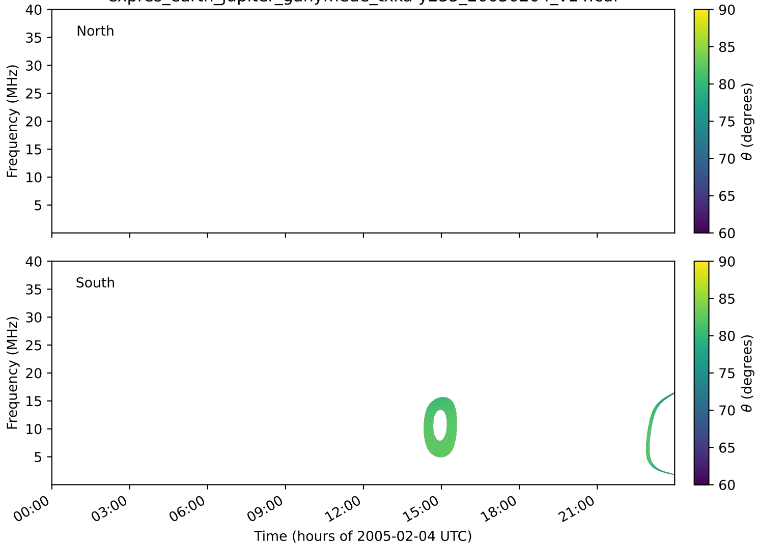
expres_earth_jupiter_ganymede_txka-y235_20050204_v14.cdf
