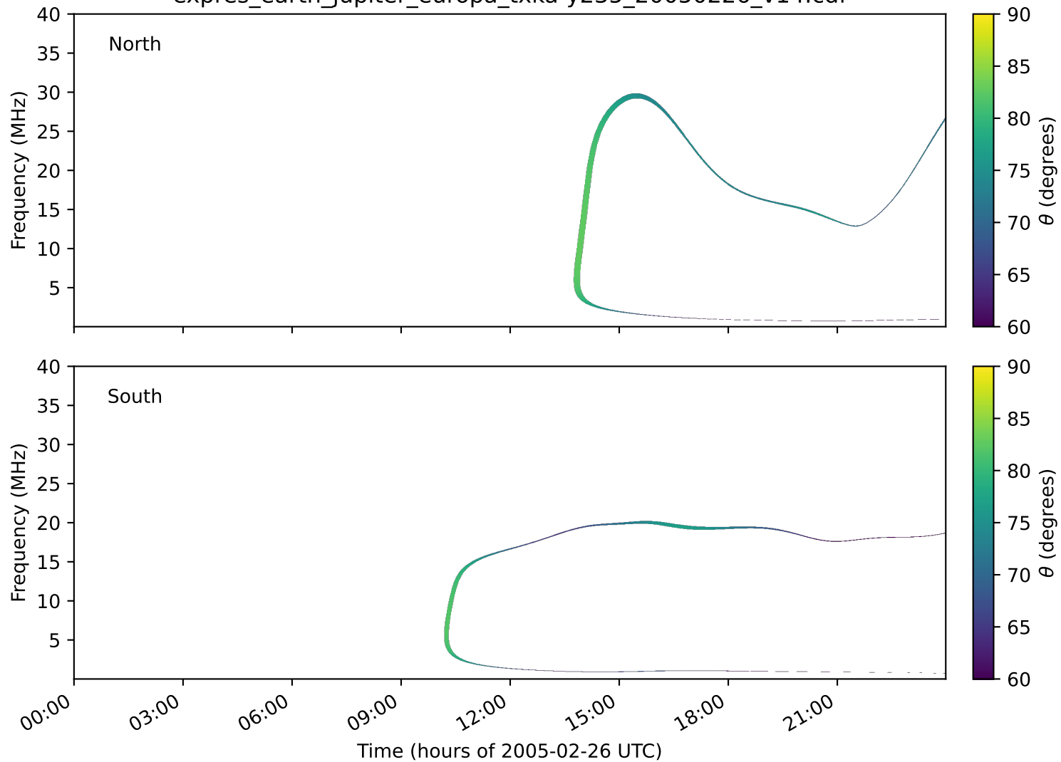
expres_earth_jupiter_europa_txka-y235_20050226_v14.cdf
