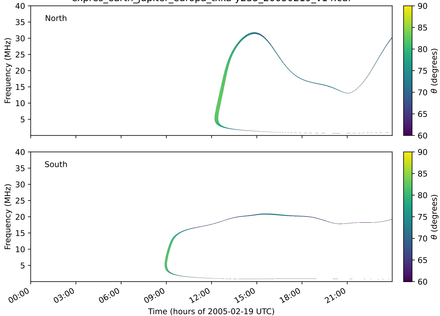
expres_earth_jupiter_europa_txka-y235_20050219_v14.cdf
