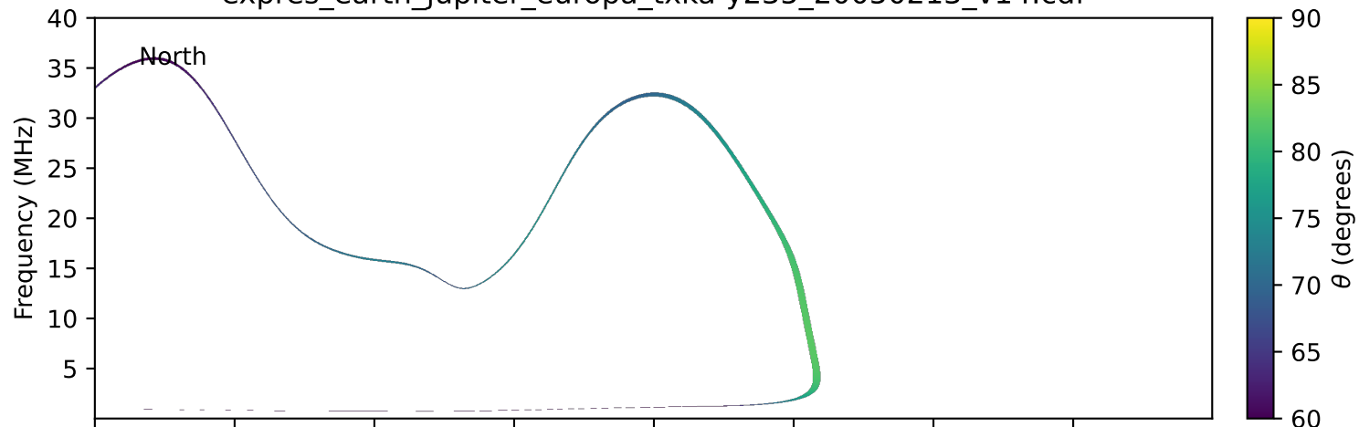
expres_earth_jupiter_europa_txka-y235_20050213_v14.cdf
