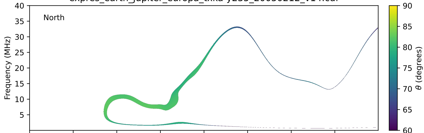
expres_earth_jupiter_europa_txka-y235_20050212_v14.cdf
