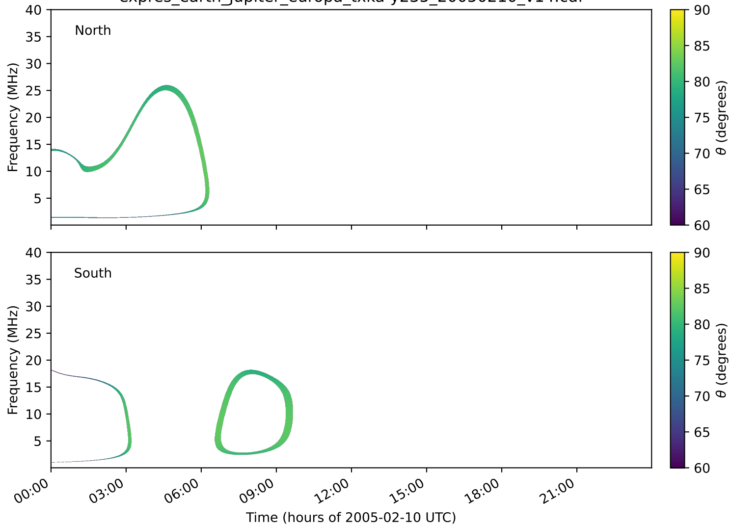
expres_earth_jupiter_europa_txka-y235_20050210_v14.cdf
