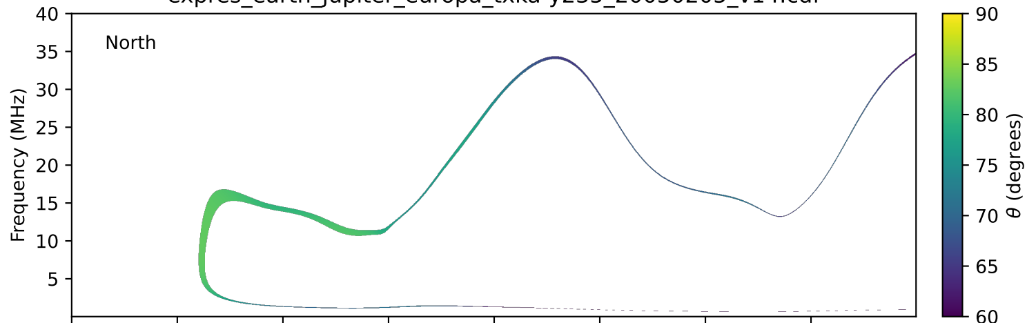
expres_earth_jupiter_europa_txka-y235_20050205_v14.cdf
