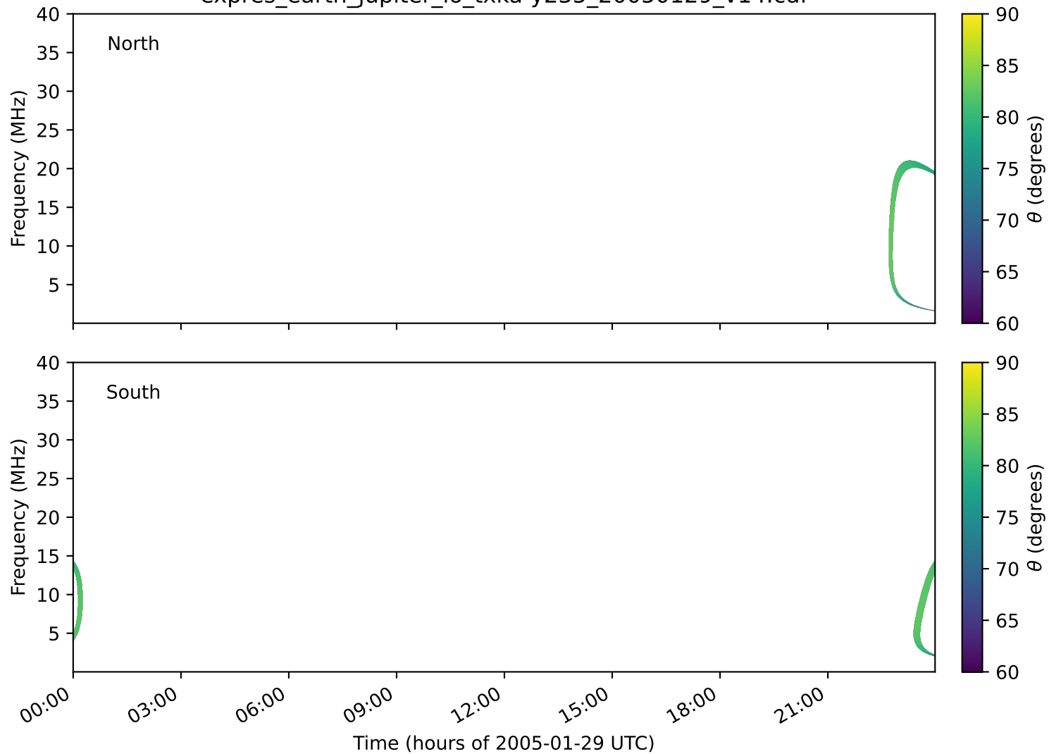
expres_earth_jupiter_io_txka-y235_20050129_v14.cdf
