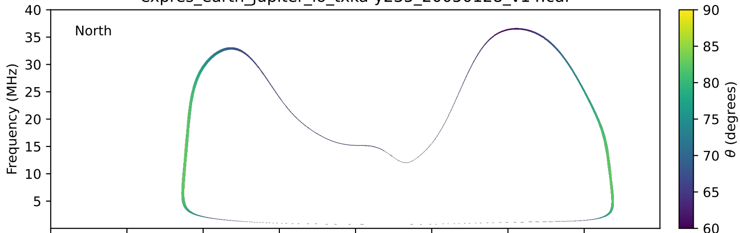
expres_earth_jupiter_io_txka-y235_20050128_v14.cdf
