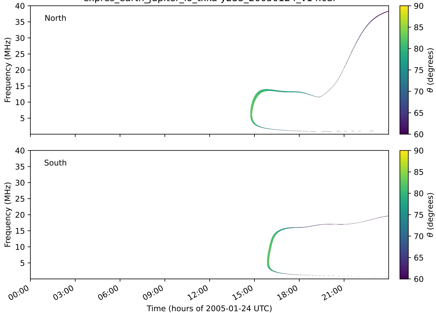
expres_earth_jupiter_io_txka-y235_20050124_v14.cdf
