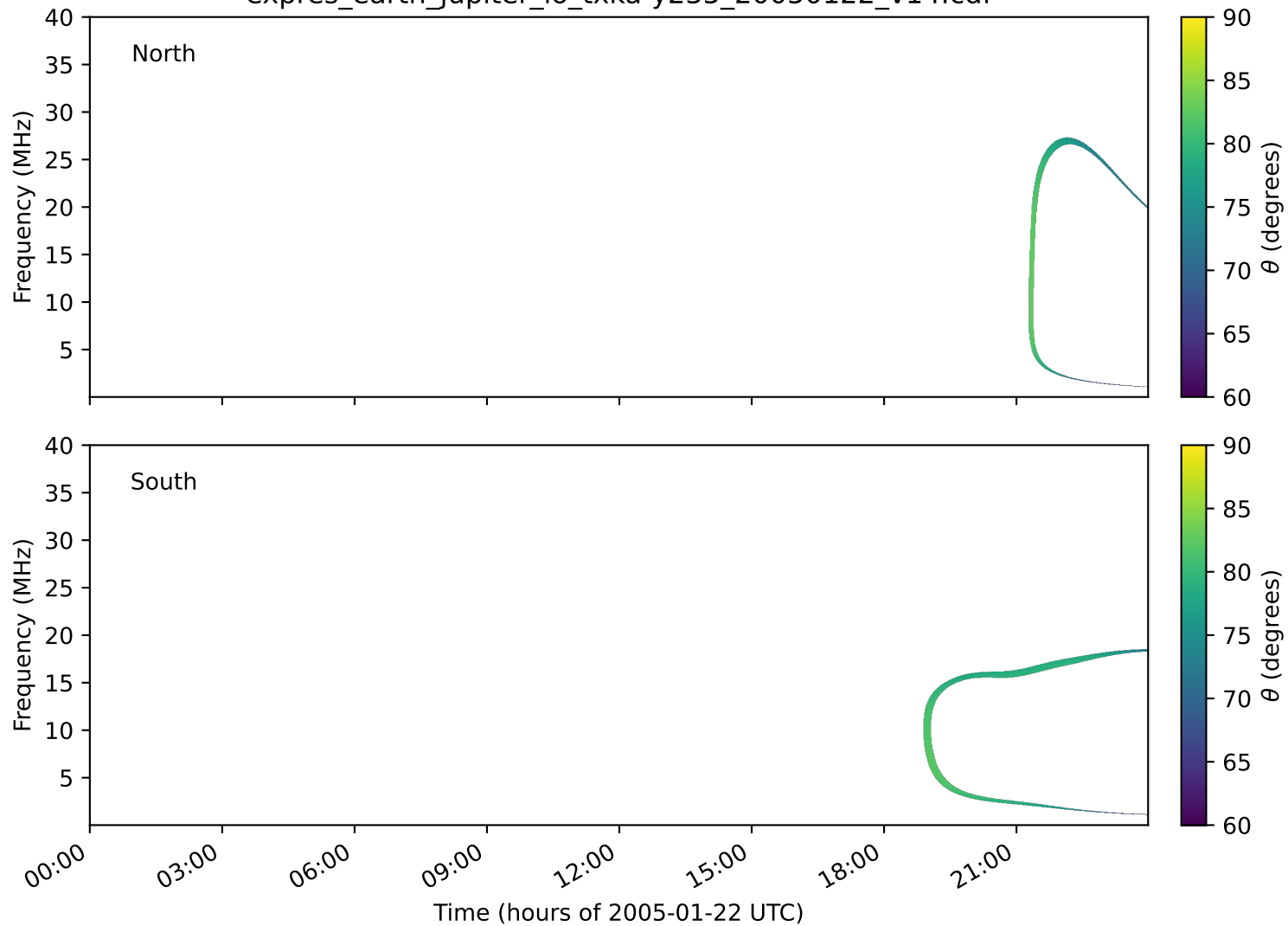
expres_earth_jupiter_io_txka-y235_20050122_v14.cdf
