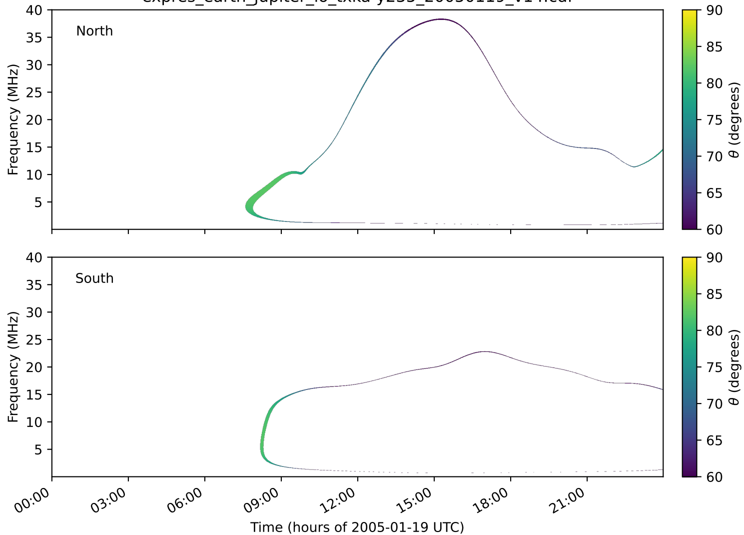
expres_earth_jupiter_io_txka-y235_20050119_v14.cdf
