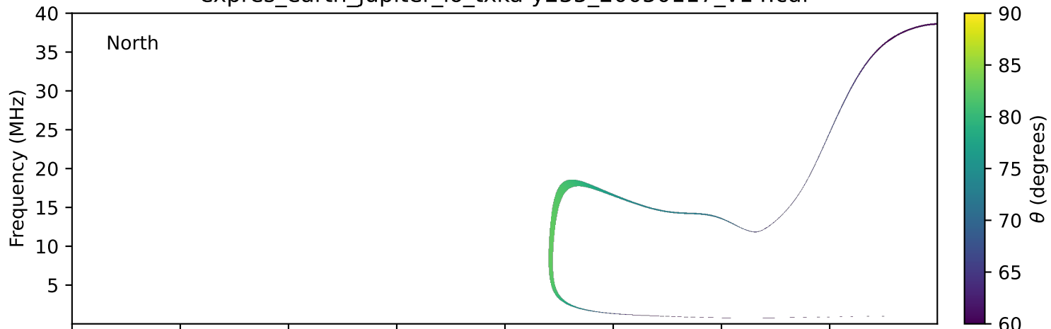
expres_earth_jupiter_io_txka-y235_20050117_v14.cdf
