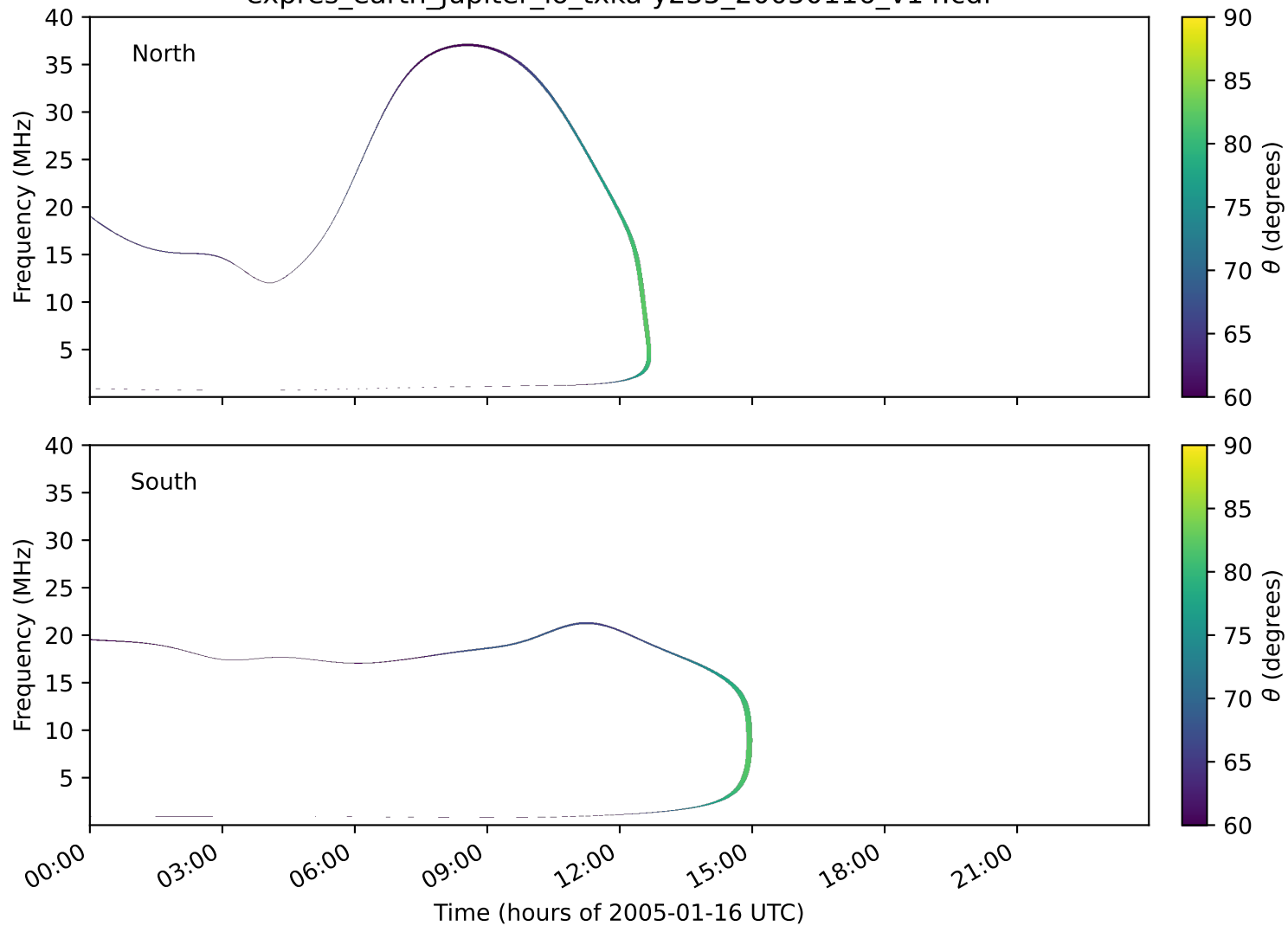
expres_earth_jupiter_io_txka-y235_20050116_v14.cdf
