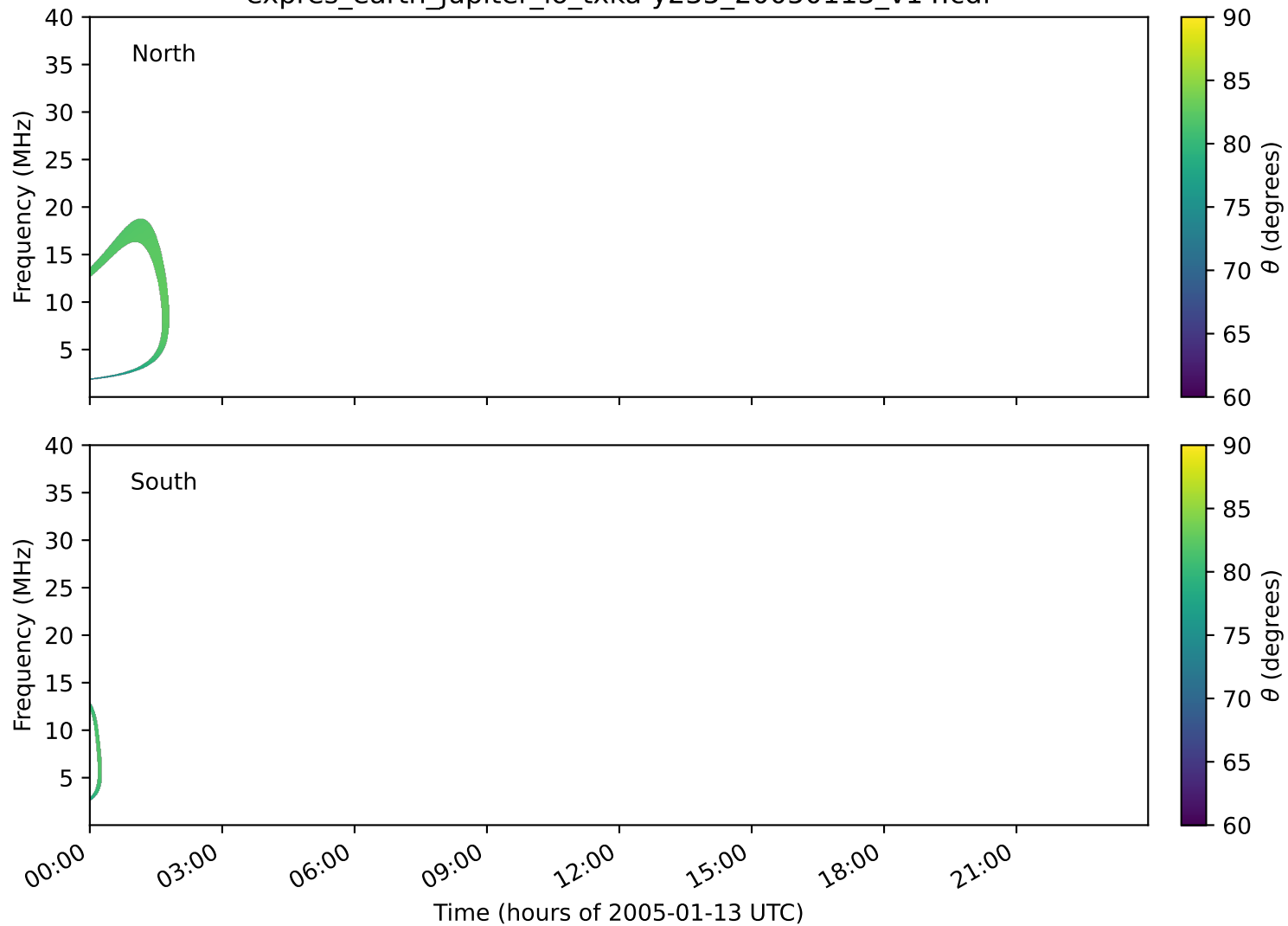
expres_earth_jupiter_io_txka-y235_20050113_v14.cdf
