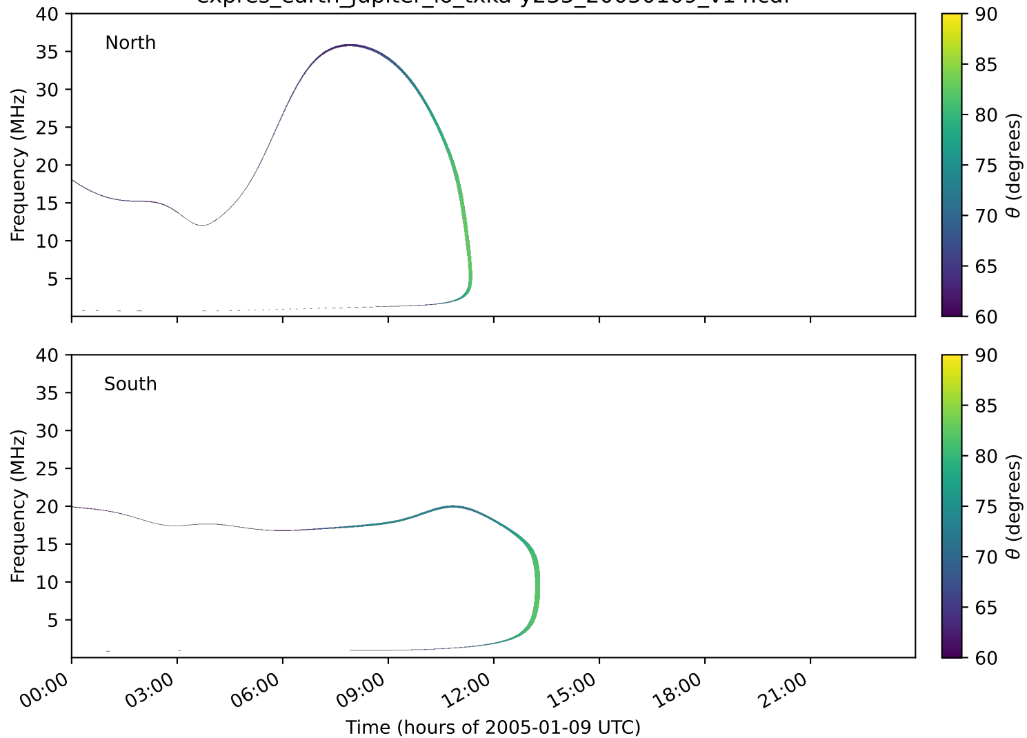
expres_earth_jupiter_io_txka-y235_20050109_v14.cdf
