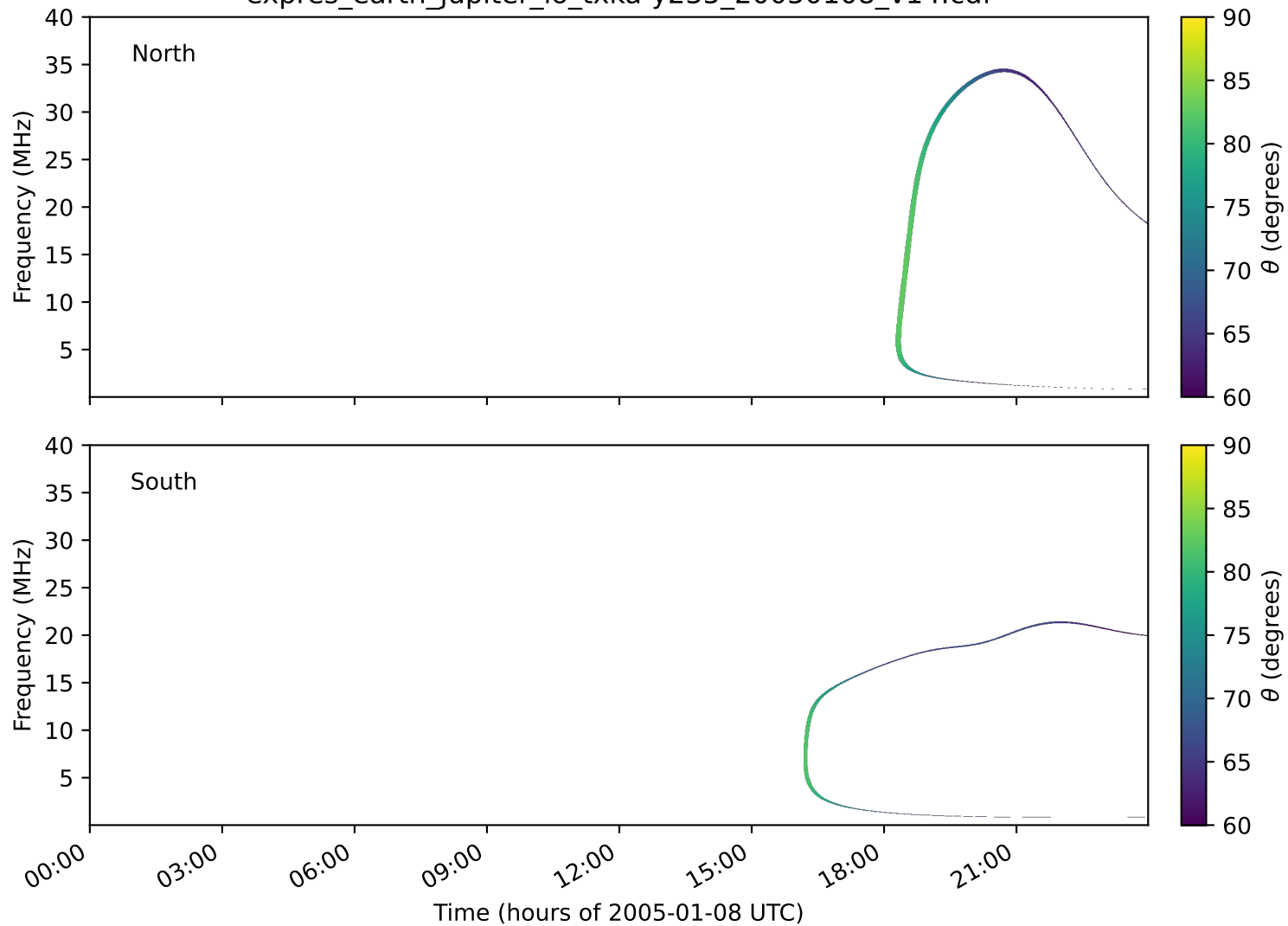
expres_earth_jupiter_io_txka-y235_20050108_v14.cdf
