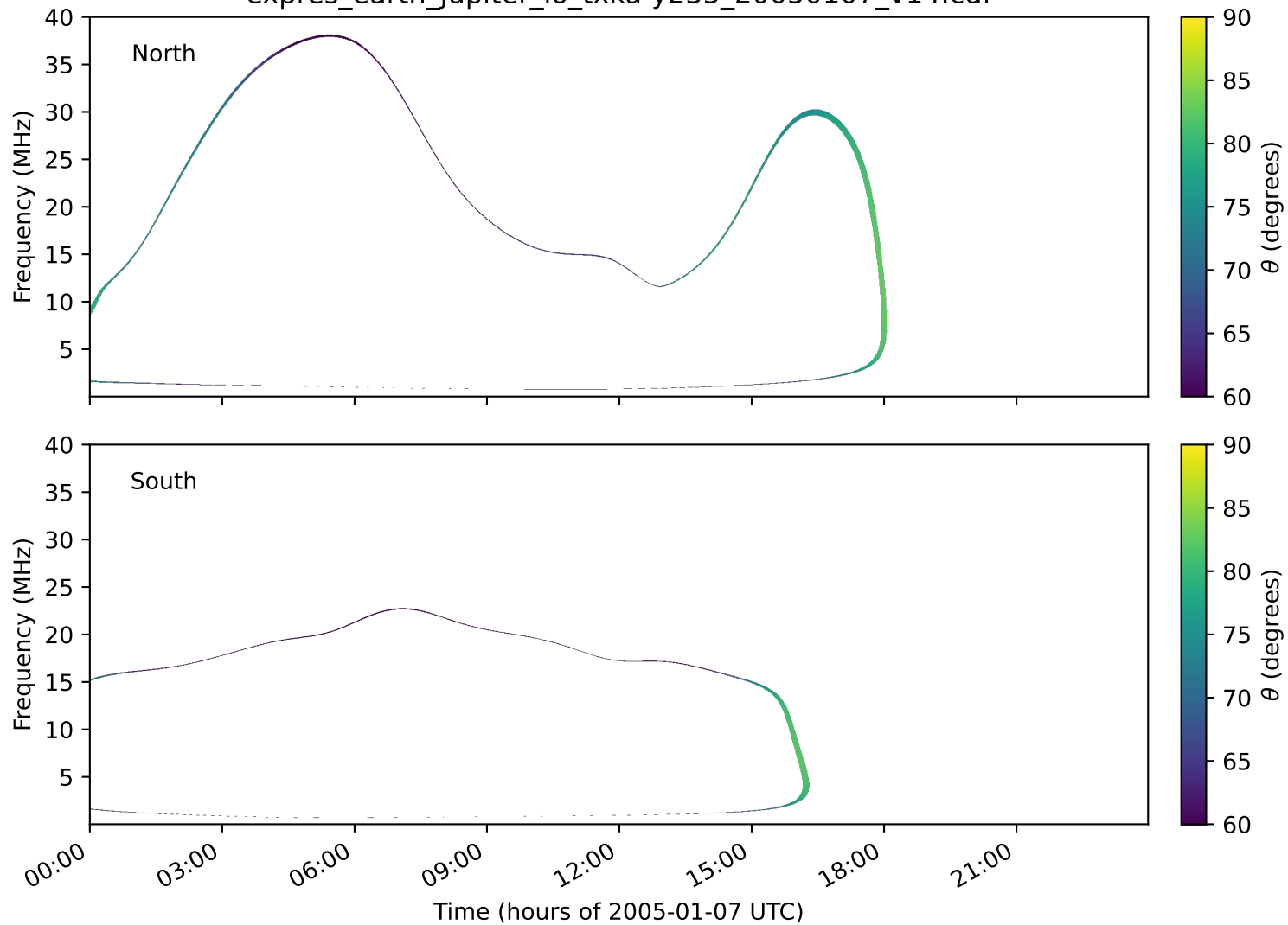
expres_earth_jupiter_io_txka-y235_20050107_v14.cdf
