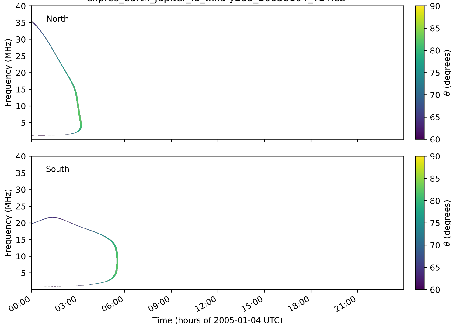
expres_earth_jupiter_io_txka-y235_20050104_v14.cdf
