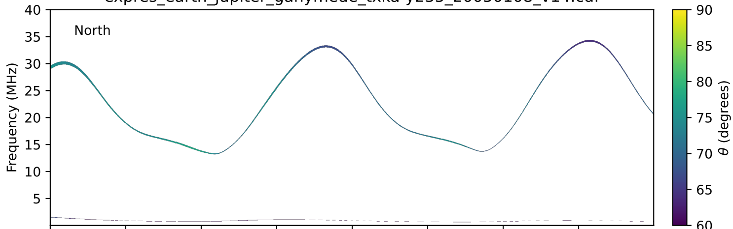
expres_earth_jupiter_ganymede_txka-y235_20050108_v14.cdf
