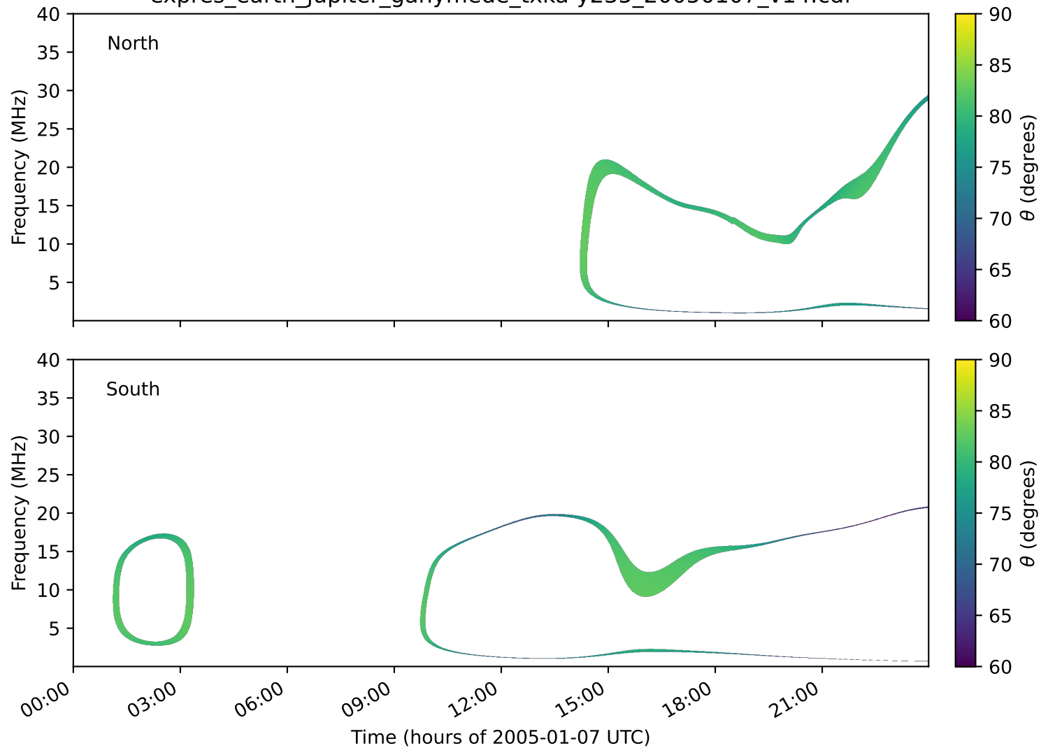
expres_earth_jupiter_ganymede_txka-y235_20050107_v14.cdf
