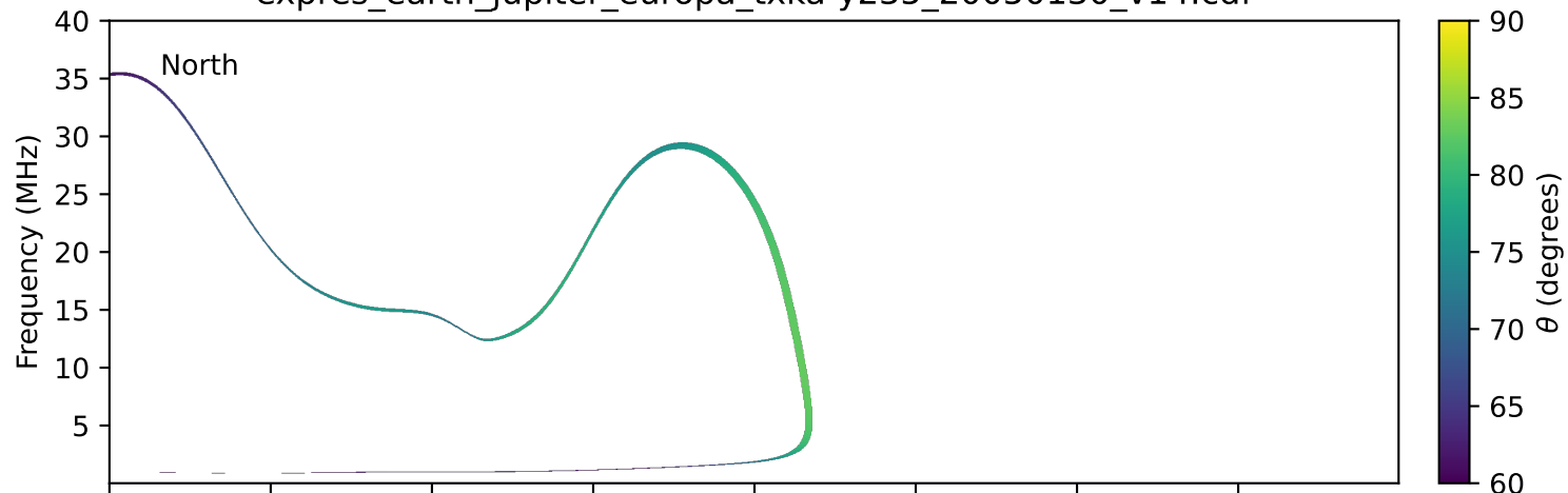
expres_earth_jupiter_europa_txka-y235_20050130_v14.cdf
