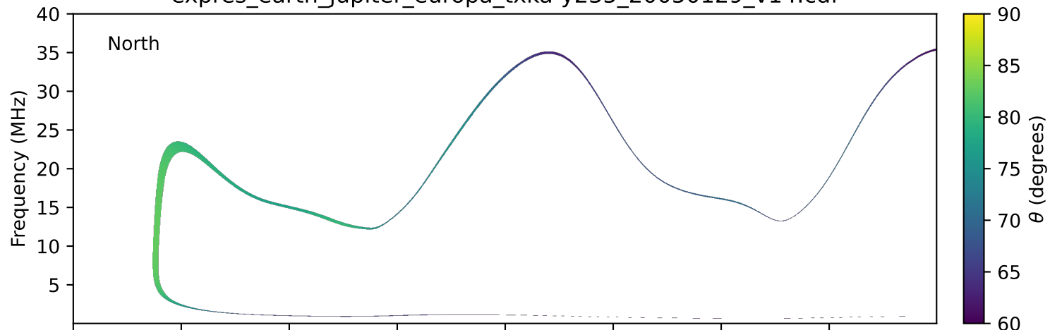
expres_earth_jupiter_europa_txka-y235_20050129_v14.cdf
