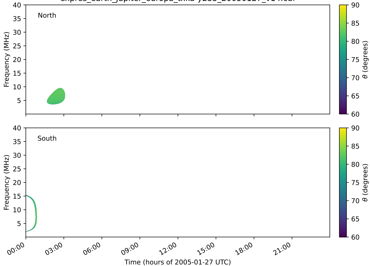
expres_earth_jupiter_europa_txka-y235_20050127_v14.cdf
