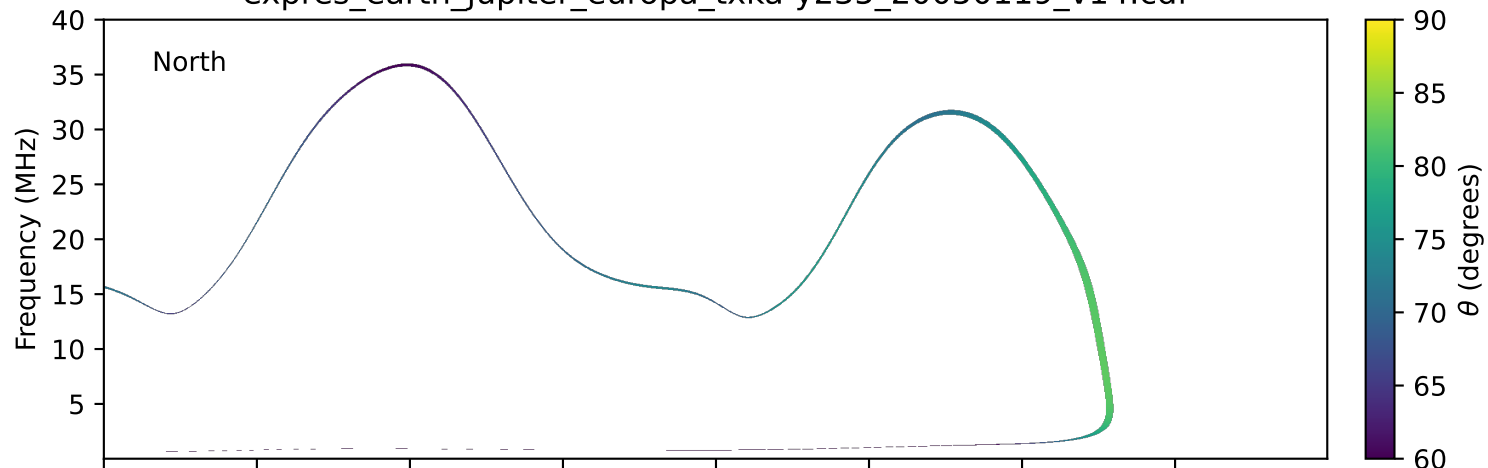
expres_earth_jupiter_europa_txka-y235_20050119_v14.cdf
