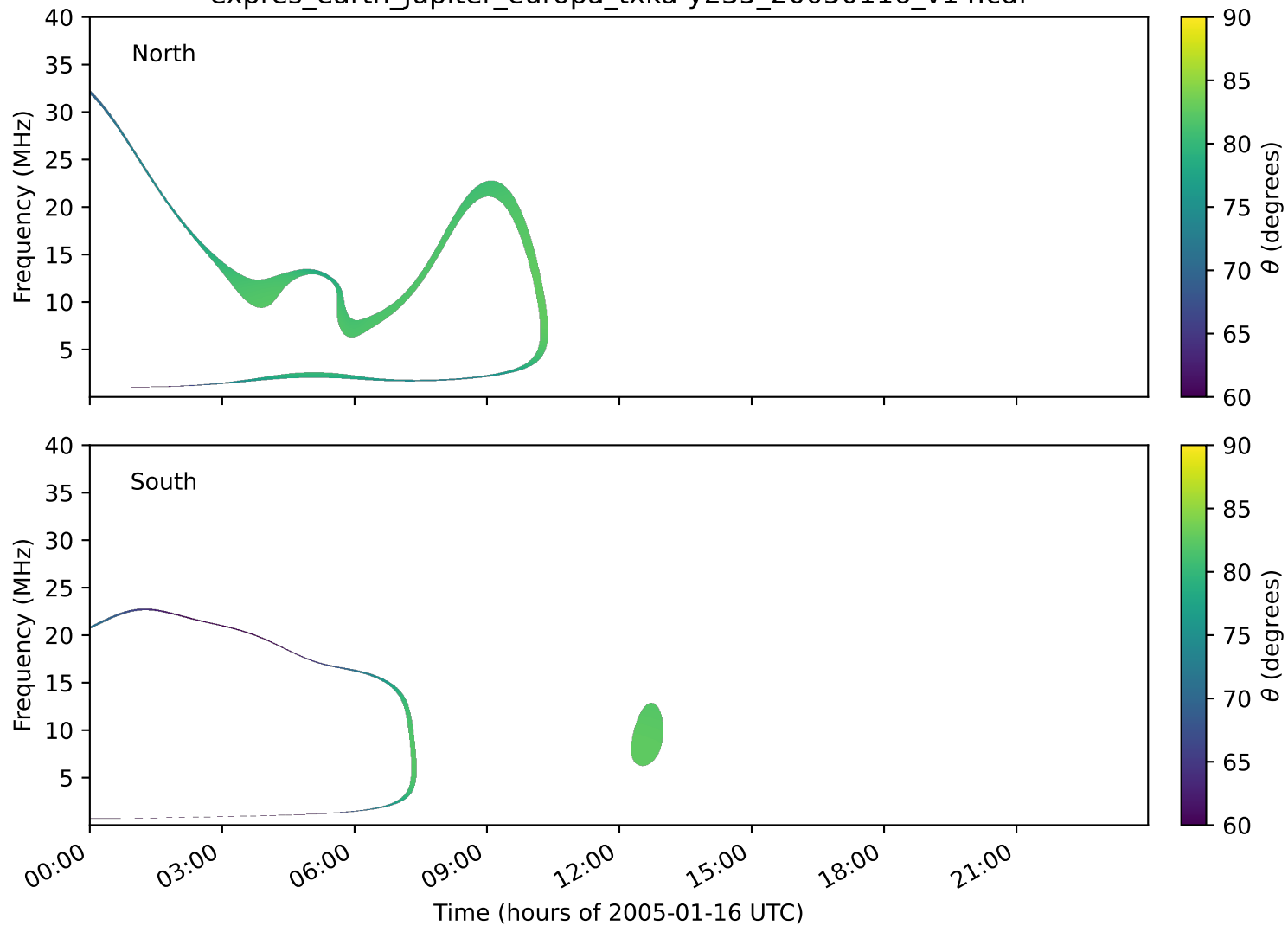
expres_earth_jupiter_europa_txka-y235_20050116_v14.cdf
