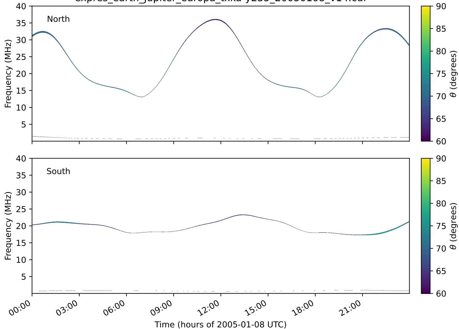
expres_earth_jupiter_europa_txka-y235_20050108_v14.cdf
