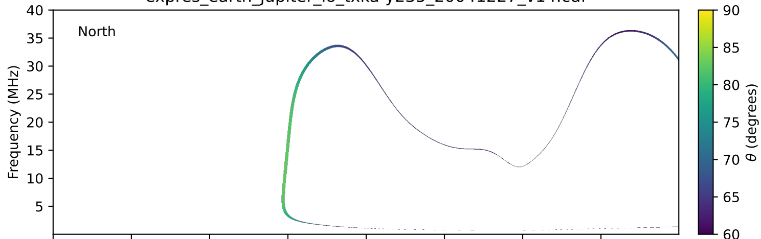
expres_earth_jupiter_io_txka-y235_20041227_v14.cdf
