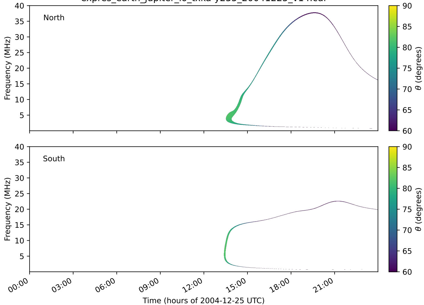
expres_earth_jupiter_io_txka-y235_20041225_v14.cdf
