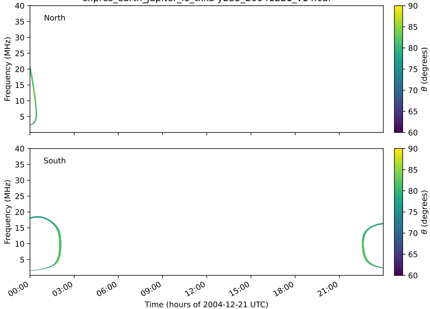
expres_earth_jupiter_io_txka-y235_20041221_v14.cdf
