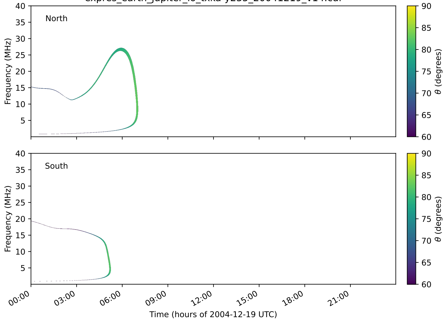
expres_earth_jupiter_io_txka-y235_20041219_v14.cdf
