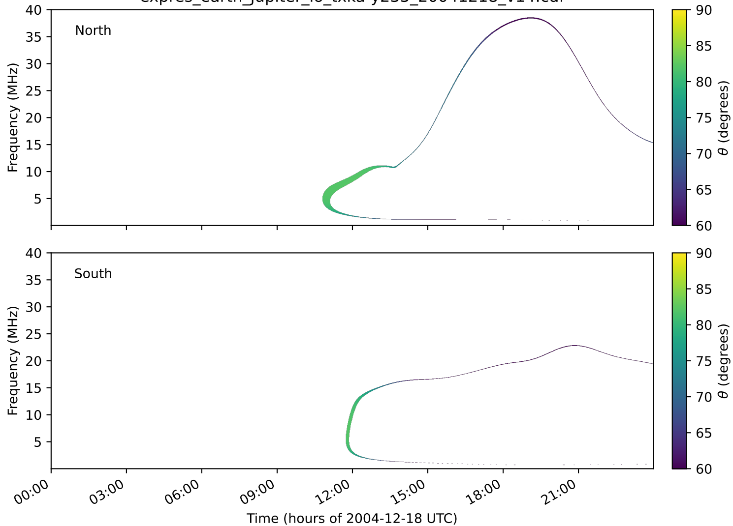
expres_earth_jupiter_io_txka-y235_20041218_v14.cdf
