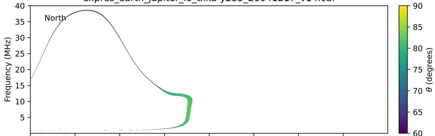
expres_earth_jupiter_io_txka-y235_20041217_v14.cdf
