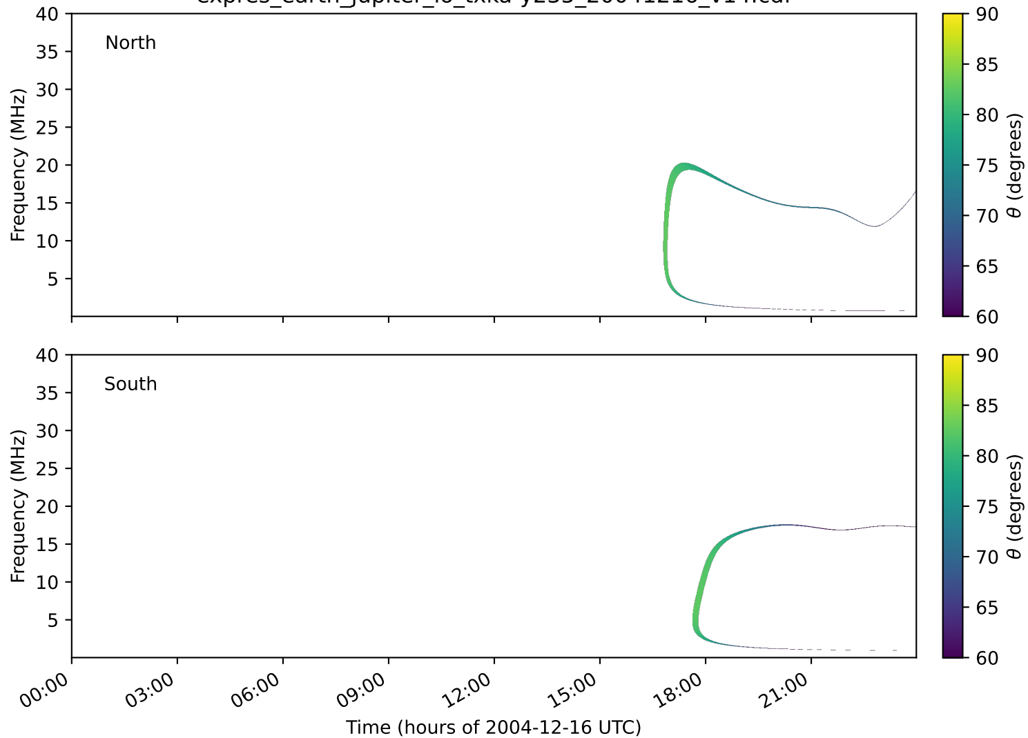
expres_earth_jupiter_io_txka-y235_20041216_v14.cdf
