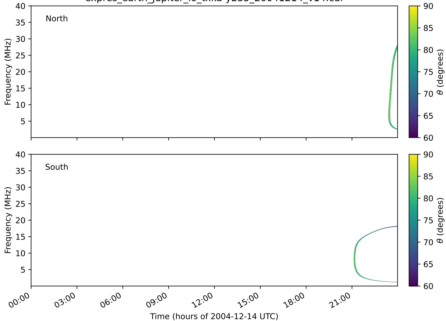
expres_earth_jupiter_io_txka-y235_20041214_v14.cdf
