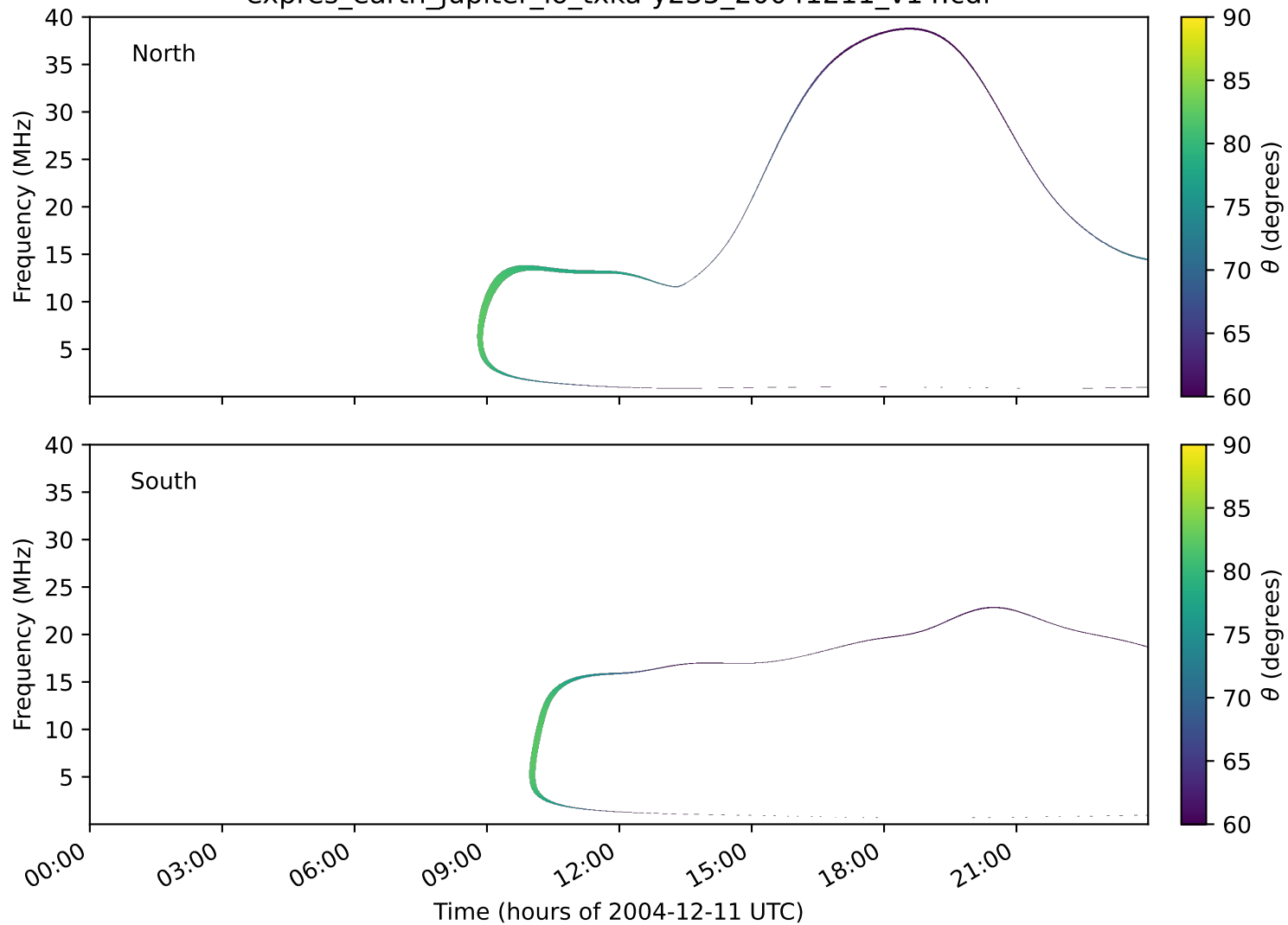
expres_earth_jupiter_io_txka-y235_20041211_v14.cdf
