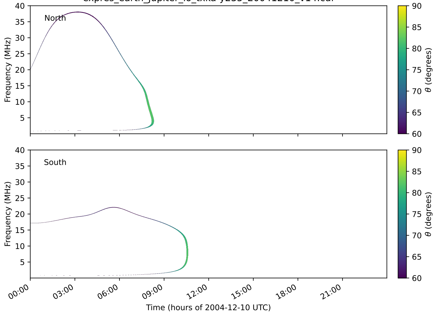
expres_earth_jupiter_io_txka-y235_20041210_v14.cdf
