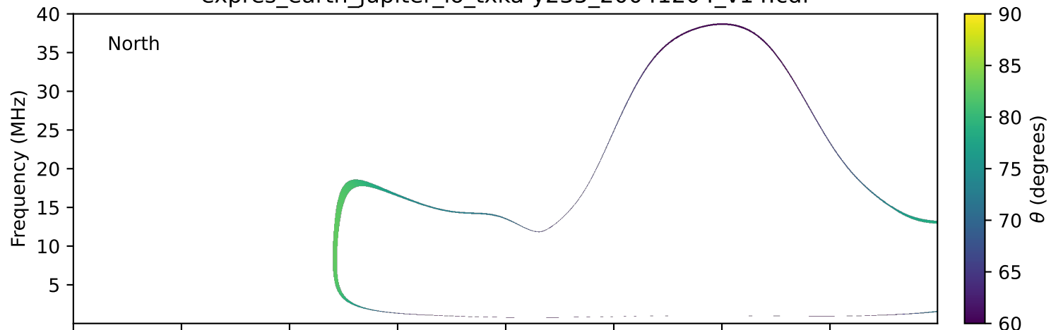
expres_earth_jupiter_io_txka-y235_20041204_v14.cdf
