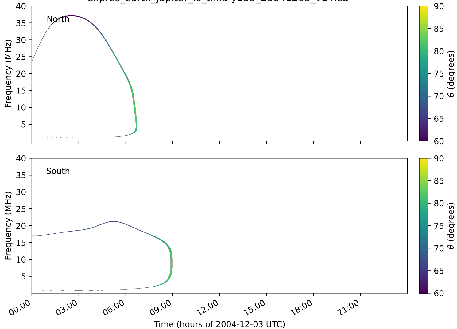
expres_earth_jupiter_io_txka-y235_20041203_v14.cdf
