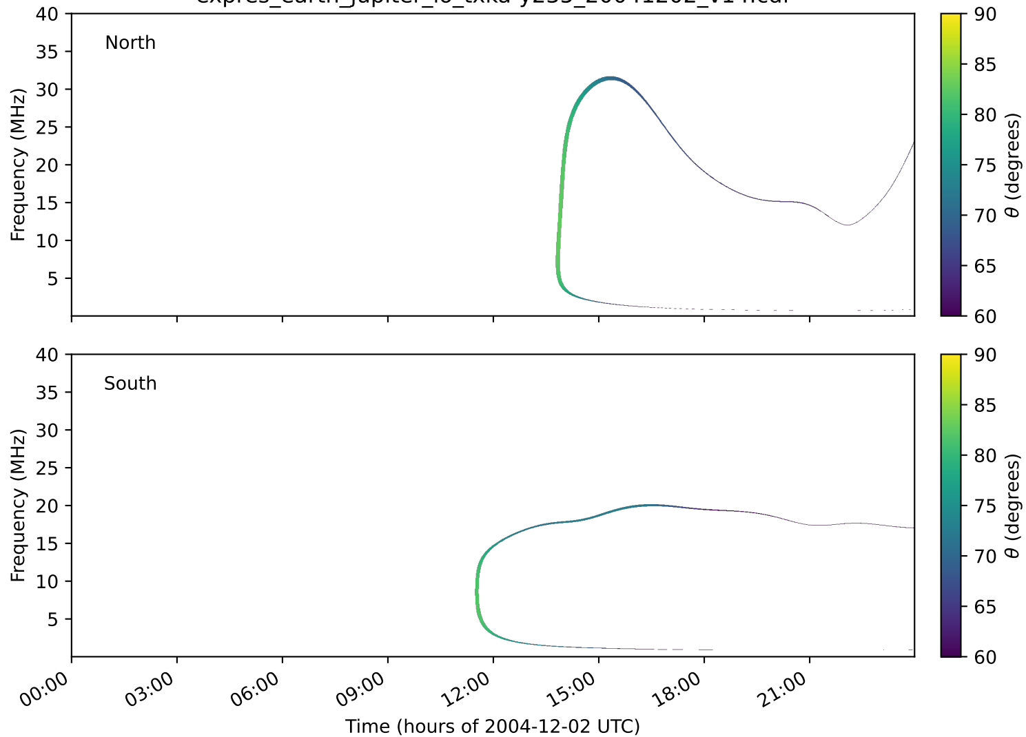
expres_earth_jupiter_io_txka-y235_20041202_v14.cdf
