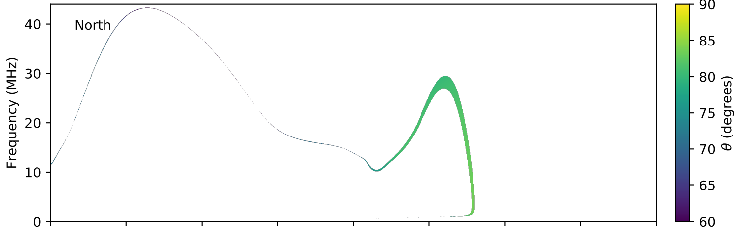
expres_earth_jupiter_io_jrm09_lossc-wid1deg_3kev_20041231_v11.cdf
