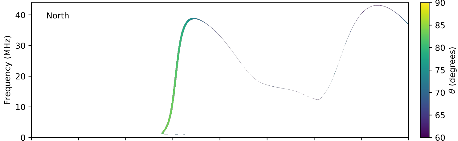
expres_earth_jupiter_io_jrm09_lossc-wid1deg_3kev_20041227_v11.cdf
