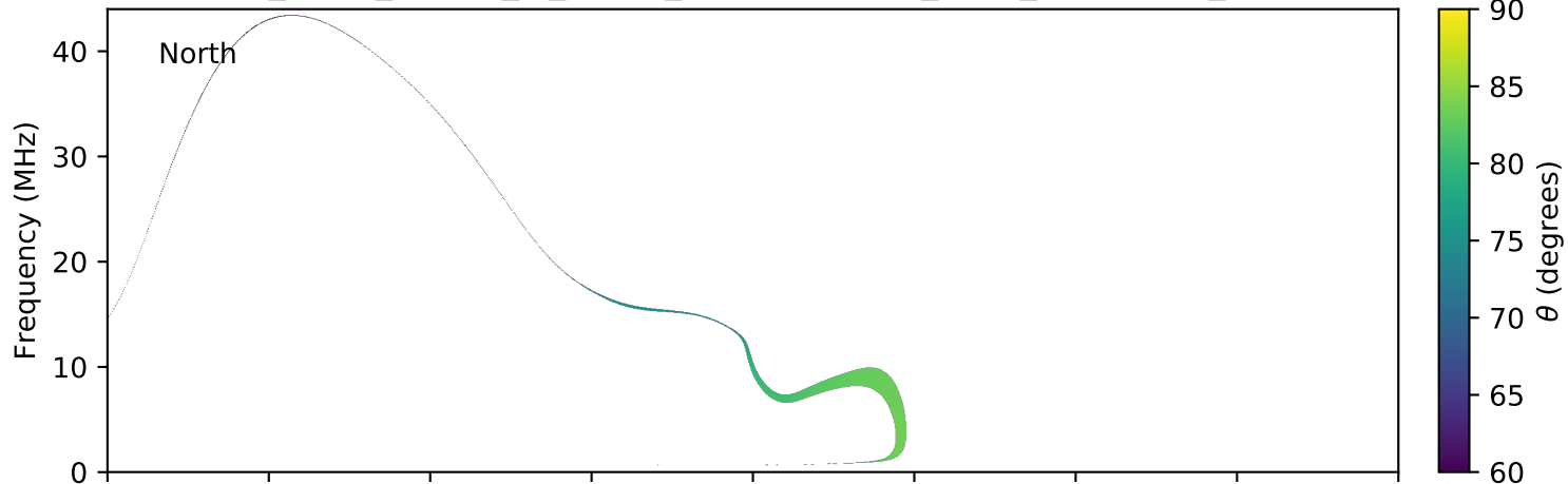
expres_earth_jupiter_io_jrm09_lossc-wid1deg_3kev_20041224_v11.cdf
