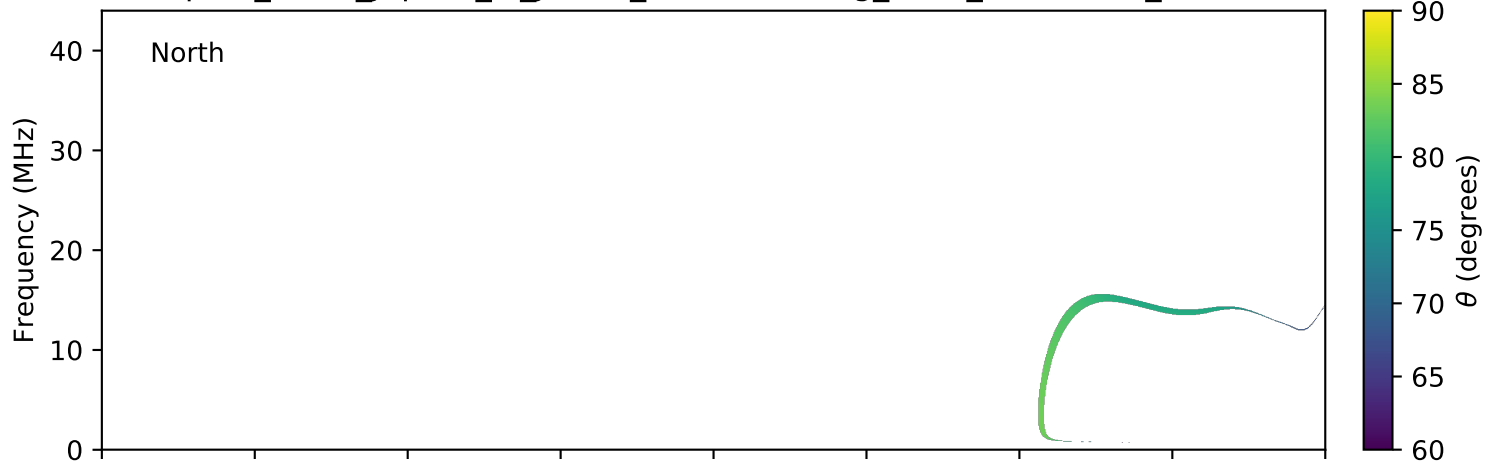
expres_earth_jupiter_io_jrm09_lossc-wid1deg_3kev_20041223_v11.cdf
